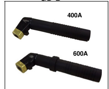
GD-B
