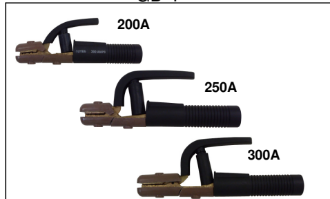
GD-T
